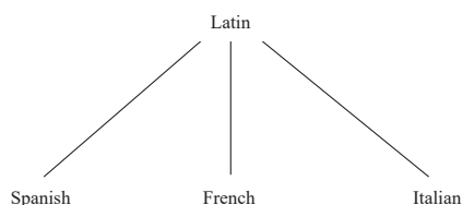
Figures 5-5 A rake (or “polytomy”)
